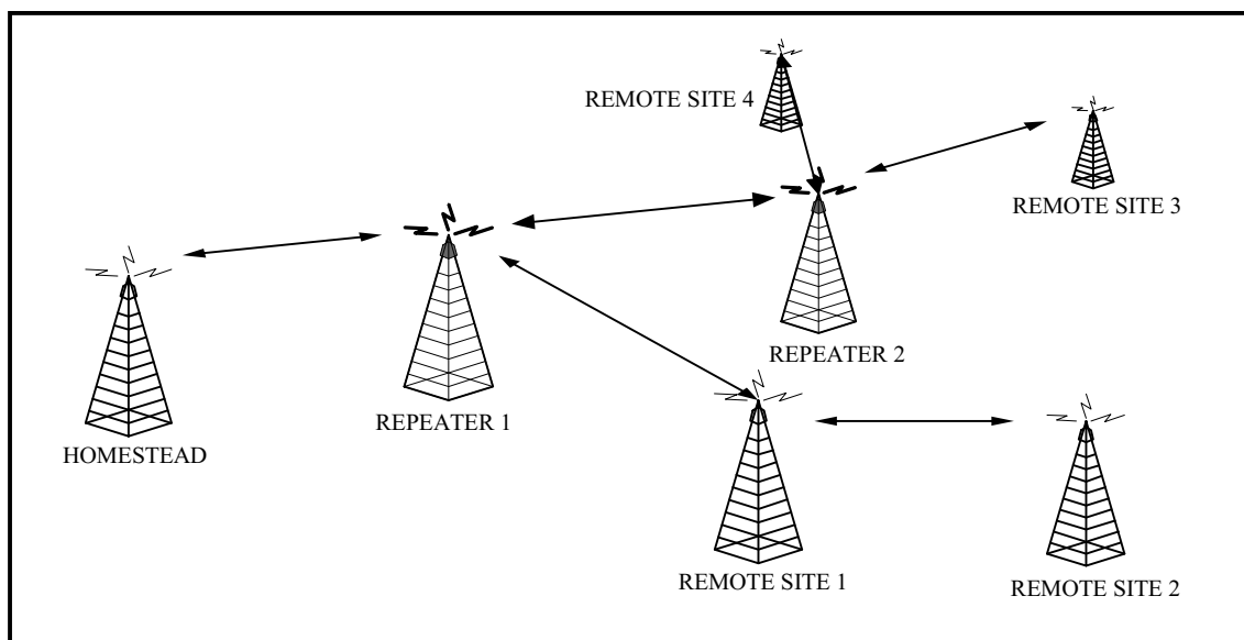
Fig. 1 A radio network topology using a remote site to also act as a repeater station (Palipana 2001).
